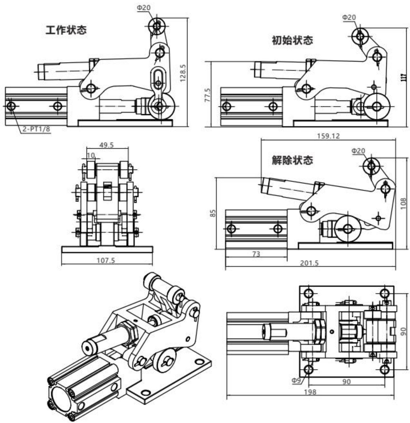
YGZX32×40-WS卧式重载阻挡气缸
