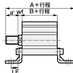
符号 通用尺寸 内螺纹时 外螺纹时 AB AD AE AG AH AK AT AU G N TR TS M WF LF 不带开关 带开关 注1 a' wf LF 不带开关 带开关 注1 A B LX AX A B LX AX A B LX AX A B LX AX φ12 6 - - 29.5 17 18 2.3 12 M4×12 15.5 16 25 6.3 3.5 8.5 38.5 17 53 41 43.5 22 58 46 10.5 3.5 8.5 49 17 53 41 54 22 58 46 φ16 6 - - 33.5 19 18 2.3 12 M4×12 20 16 29 6.3 3.5 8.5 38.5 17 53 41 43.5 22 58 46 12 3.5 8.5 50.5 17 53 41 55.5 22 58 46 φ20 7 - - 42 24 24 3.2 16 M6×16 25.5 24 36 9.2 4.5 11.5 48 19.5 67.5 51.5 58 29.5 77.5 61.5 14 4.5 11.5 62 19.5 67.5 51.5 72 29.5 77.5 61.5 φ25 7 - - 46 26 24 3.2 16 M6×16 28 28 40 9.2 5 11 51.5 22.5 70.5 54.5 61.5 32.5 80.5 64.5 17.5 5 11 69 22.5 70.5 54.5 79 32.5 80.5 64.5 φ32 7 - - 53.5 31 24 3.2 16 M6×16 34 34 45 9.2 7 9 54 23 71 55 64 33 81 65 23.5 5 11 75.5 23 71 55 85.5 33 81 65 φ40 7 26 20 71 40 29 4.5 19 M6×16 40 40 52 10 7 12 65.5 29.5 87.5 67.5 75.5 39.5 97.5 77.5 23.5 5 14 87 29.5 87.5 67.5 97 39.5 97.5 77.5 φ50 9 23 15 79 40 34 4.5 22 M8×20 50 46 64 13 8 14 72.5 30.5 98.5 74.5 82.5 40.5 108.5 84.5 28.5 5 17 98 30.5 98.5 74.5 108 40.5 108.5 84.5 φ63 11 33 21 96.5 51 40 4.5 25 M10×25 60 60 77 15 8 17 84 36 116 86 94 46 126 96 28.5 5 20 108.5 36 116 86 119.5 46 126 96 φ80 13 42 23 116.5 61.5 50 6 35 M12×40 77 77 98 18 10 25 103.5 43.5 143.5 113.5 113.5 53.5 153.5 123.5 35.5 8 27 137 43.5 143.5 113.5 147 53.5 153.5 123.5 φ100 13 48 22 134 69 50 6 35 M12×40 94 94 117 18 12 23 115 53 153 123 125 63 163 133 35.5 8 27 146.5 53 153 123 156.5 63 163 133
