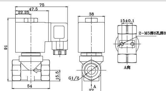
YCSM41-1/2G(N) Coil : S21B Material: stainless steel / brass
